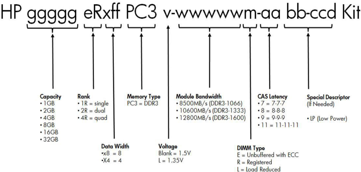
DDR3 memory options part number decoder
